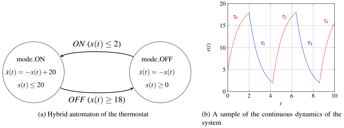
Figure 1: Thermostat example
