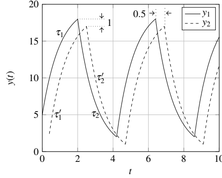
Figure 2: Two signals which are \approx_{\tau, \varepsilon} for \tau = 0.4 and \varepsilon = 0.8 but not for \tau = 1 and \varepsilon = 0.8 .
